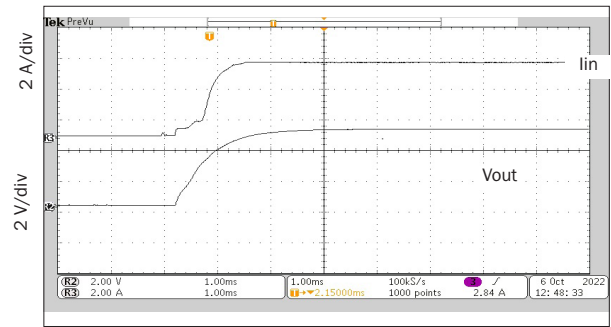
1 ms/div rMOR2805S INHIBIT RELEASE INRUSH CURRENT
