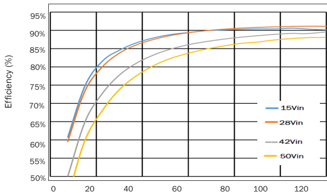
OUTPUT POWER (Watts) rMOR2812S Efficiency FIGURE 14
