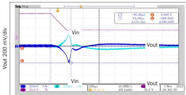
100 μs/div 50 to 15 V rMOR2815D STEP LINE RESPONSE FIGURE 33
