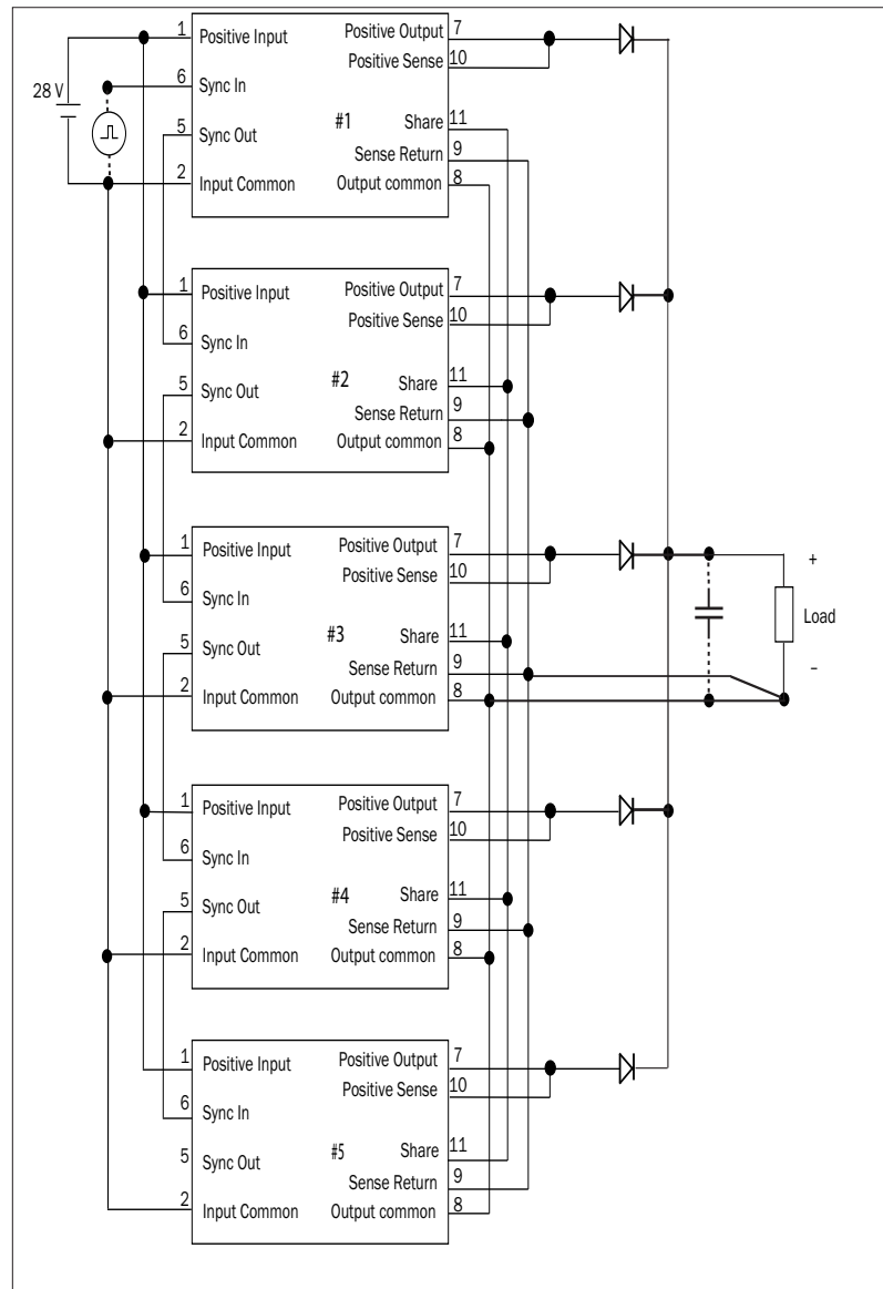
FIGURE 5: PARALLELING
