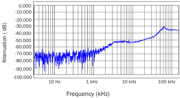
Frequency (kHz) rMOR2805S Audio Rejection FIGURE 18
