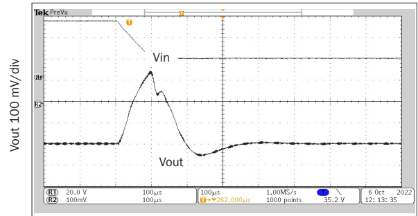
100 μs/div 50 to 15 V rMOR2805S STEP LINE RESPONSE
