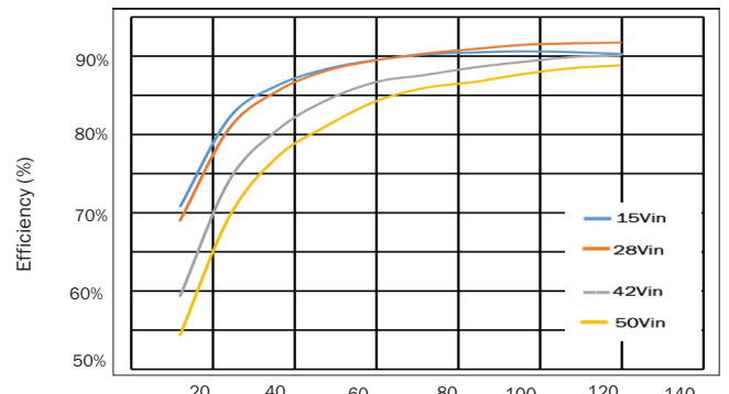
OUTPUT POWER (Watts) rMOR2815D Efficiency FIGURE 17
