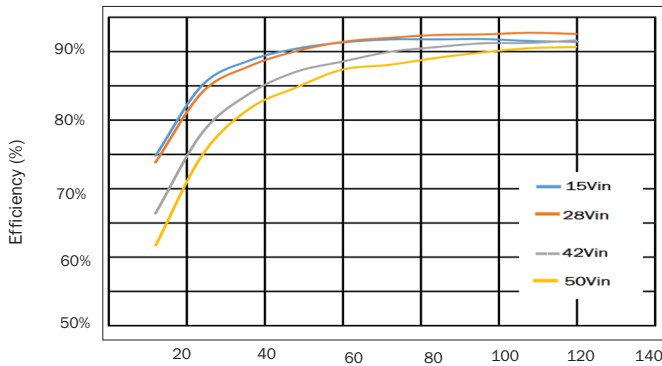
OUTPUT POWER (Watts) rMOR2812D Efficiency FIGURE 16
