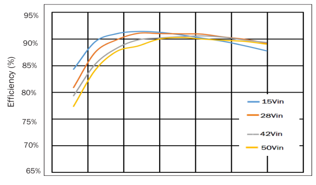
OUTPUT POWER (Watts) rMOR2805D Efficiency FIGURE 15
