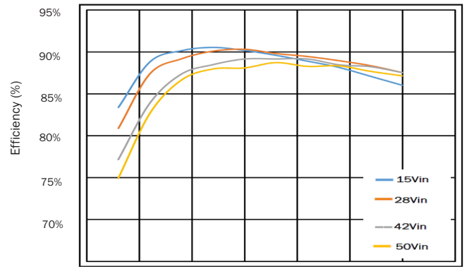
OUTPUT POWER (Watts) rMOR2805S Efficiency FIGURE 13
