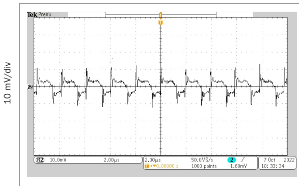
2 µs/div rMOR2805S Output Ripple (Vout) FIGURE 20
