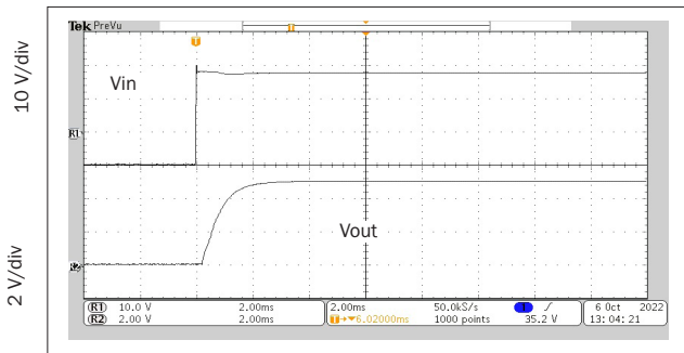
2 ms/div All combinations of line and load rMOR2805S START-UP RESPONSE
