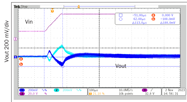
100 μs/div 15 to 50 V rMOR2815D STEP LINE RESPONSE FIGURE 32
