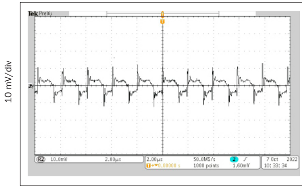
2 μs/div (PLACE HOLDER PENDING) rMOR2815D Output Ripple (Vout) FIGURE 29
