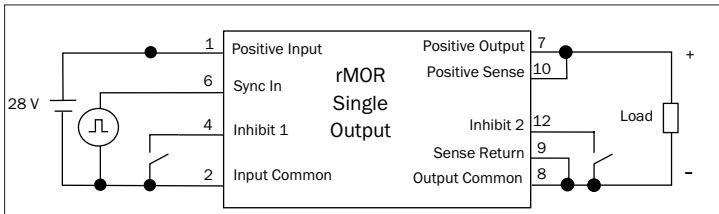
FIGURE 6: TYPICAL CONNECTIONS WITH SENSE PIN
