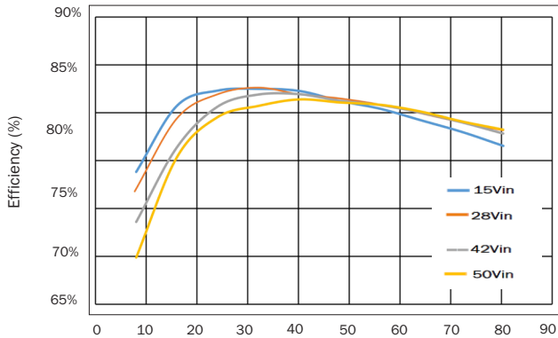
OUTPUT POWER (Watts) rMOR283R3S Efficiency FIGURE 12
