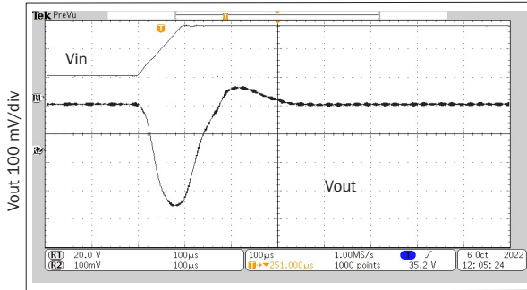
100 μs/div 15 to 50 V rMOR2805S STEP LINE RESPONSE
