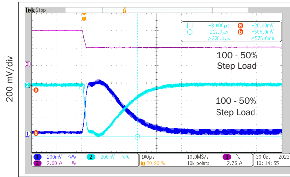
100 μs/div 100% to 50% Load rMOR2815D STEP LOAD RESPONSE FIGURE 30
