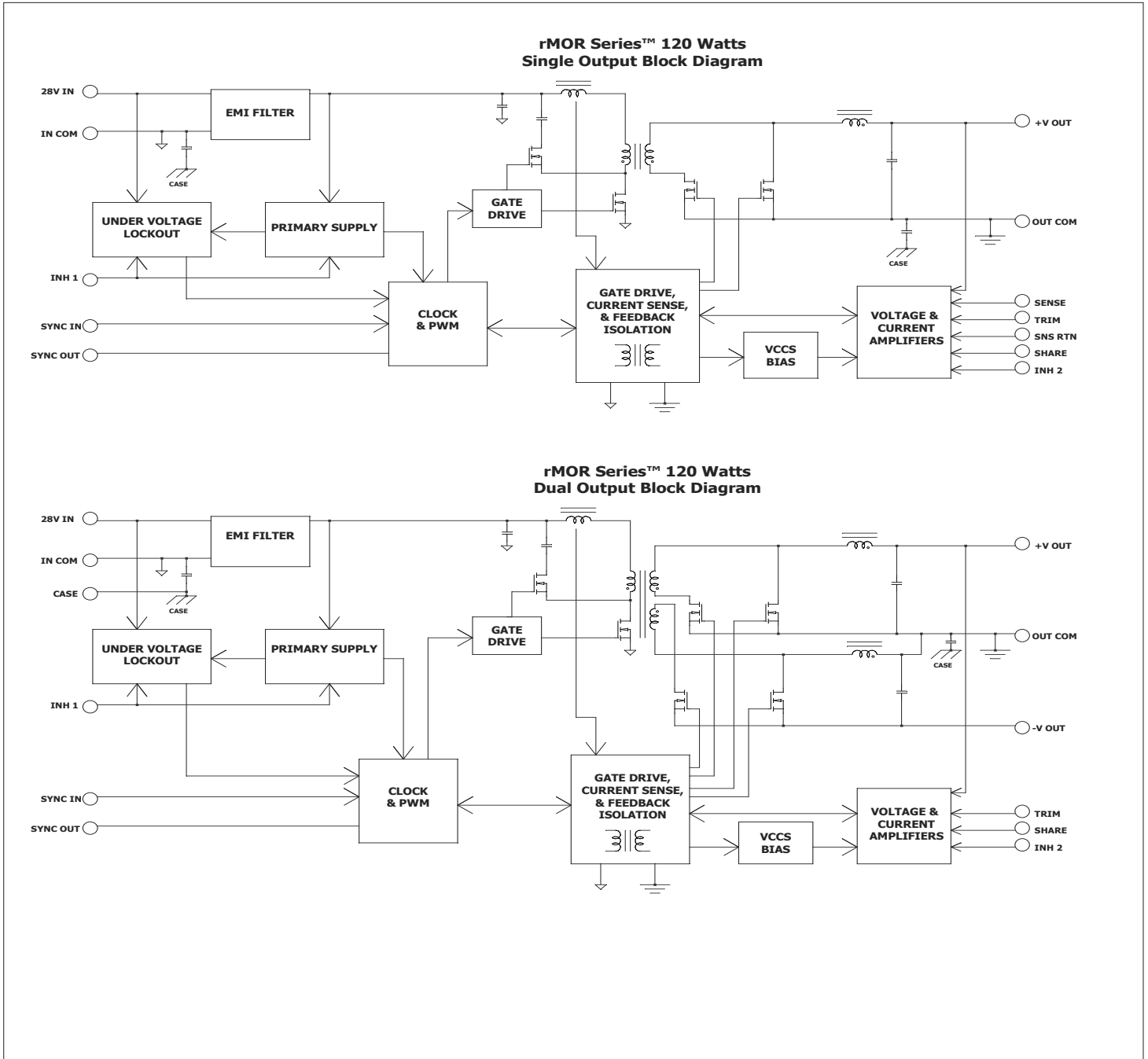
FIGURE 9: RMOR SINGLE AND DUAL OUTPUT BLOCK DIAGRAM
