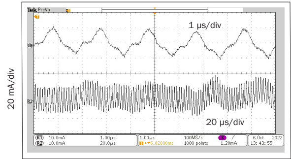
rMOR2805S Input Ripple Current (Iin) FIGURE 19
