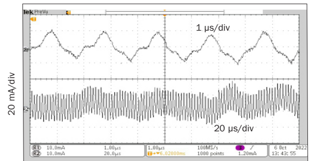
(PLACE HOLDER PENDING) rMOR2815D Input Ripple Current (Iin)
