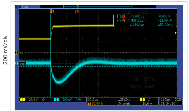
200 µs/div 50% to 100% Load rMOR2805S STEP LOAD RESPONSE FIGURE 22
