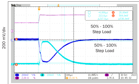
100 μs/div 50% to 100% Load rMOR2815D STEP LOAD RESPONSE FIGURE 31
