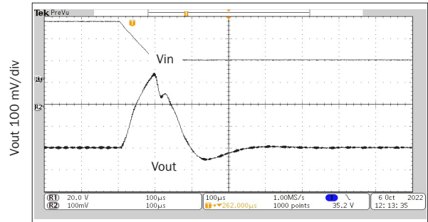
100 μs/div 50 to 15 V cMOR2805S STEP LINE RESPONSE
