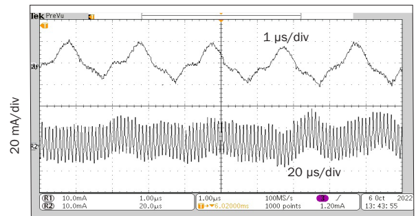
(PLACE HOLDER_PENDING) rMOR2815D Input Ripple Current (lin)
