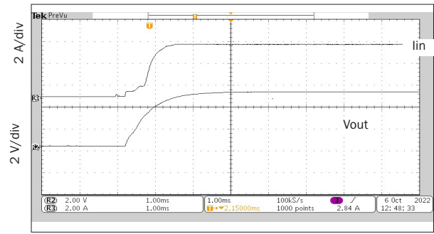
1 ms/div cMOR2805S INHIBIT RELEASE INRUSH CURRENT
