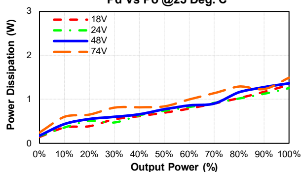
EC2SBW-48D15H Pd Vs Po @25 Deg. C
